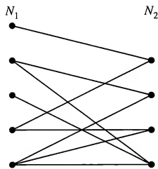
FIGURE 8.10-2 A bipartite graph.
