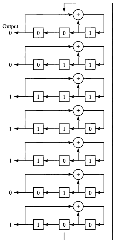
FIGURE 7.9-9 The seven states for the m = 3 maximum-length shift register.
