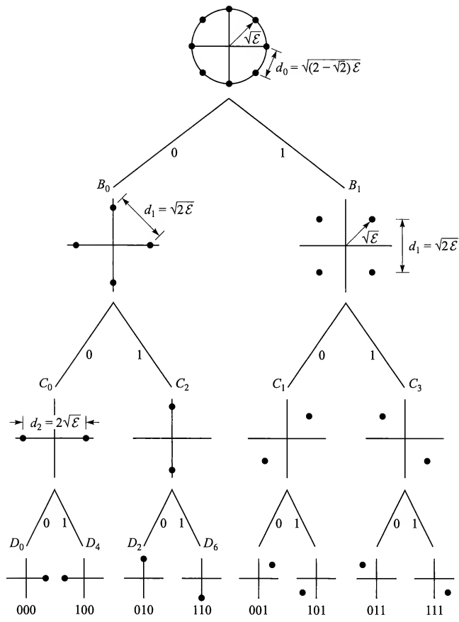
FIGURE 8.12-1 Set partitioning of an 8-PSK signal set.
