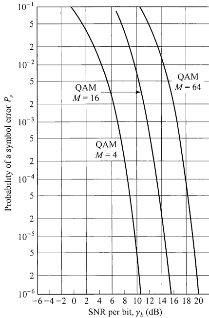
FIGURE 4.3-8 Probability of a symbol error for QAM.
