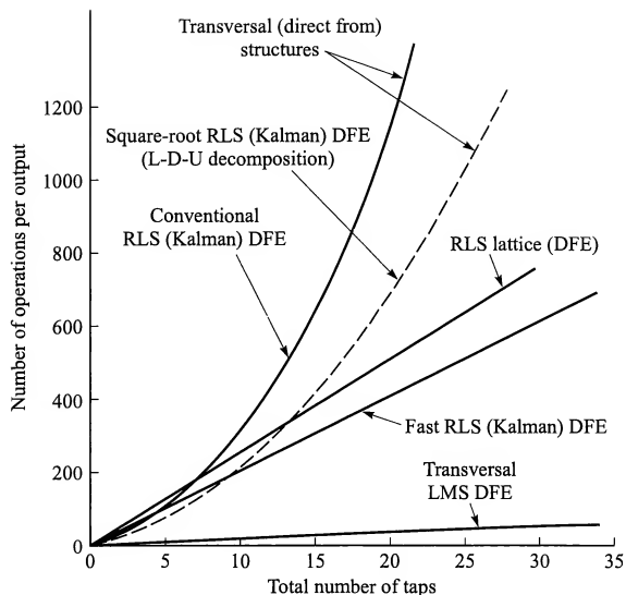
FIGURE 10.4-3 Computational complexity of DFE algorithms.
