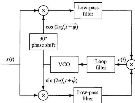
FIGURE 5.2–15 Block diagram of Costas loop.
