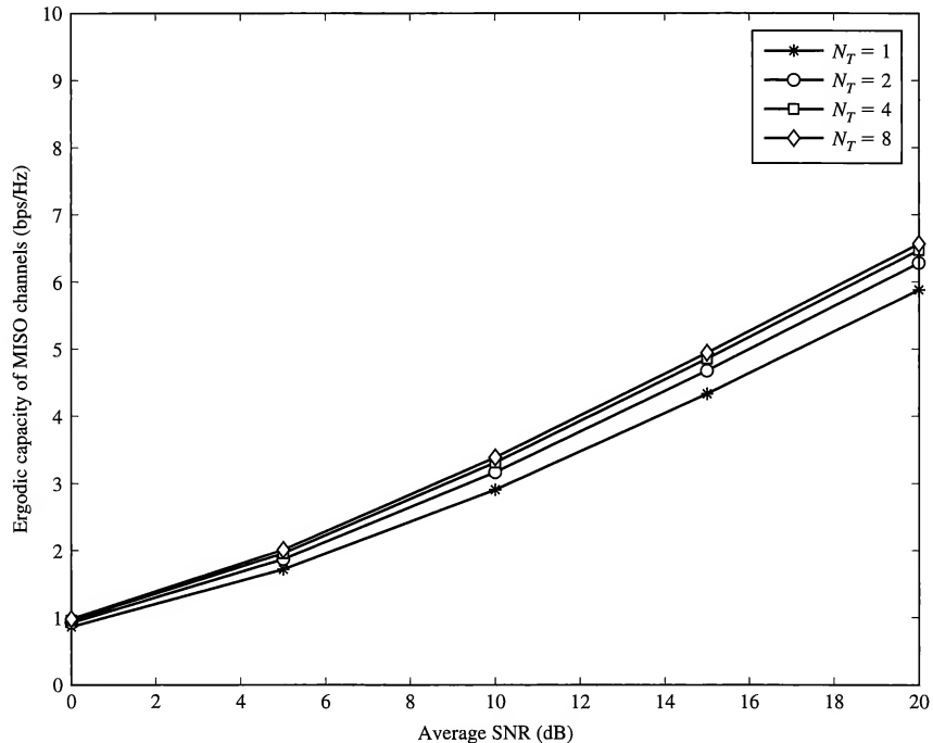
FIGURE 15.2–2 Ergodic capacity of MISO channels.
