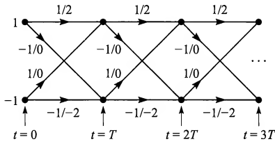
FIGURE 9.2-12 Trellis for duobinary partial-response signal.
