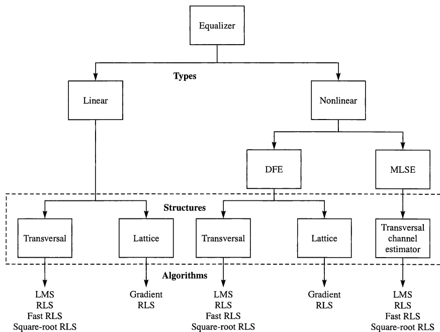
FIGURE 10.4-4 Equalizer types, structures, and algorithms.
