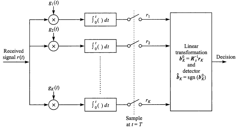
FIGURE 16.3–2 Receiver structure for decorrelation receiver.
