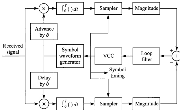
FIGURE 5.3-5 Block diagram of early-late gate synchronizer.
