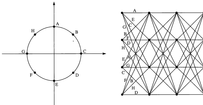
FIGURE 14.5–1 A TCM scheme for fading channels.
