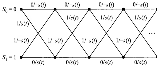
FIGURE 3.3-3 The trellis diagram for NRZI signaling.
