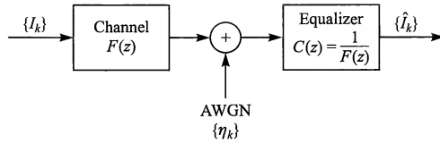
FIGURE 9.4-2 Block diagram of channel with zero-forcing equalizer.
