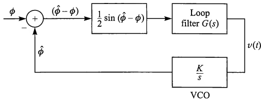
FIGURE 5.2-4 Model of phase-locked loop.
