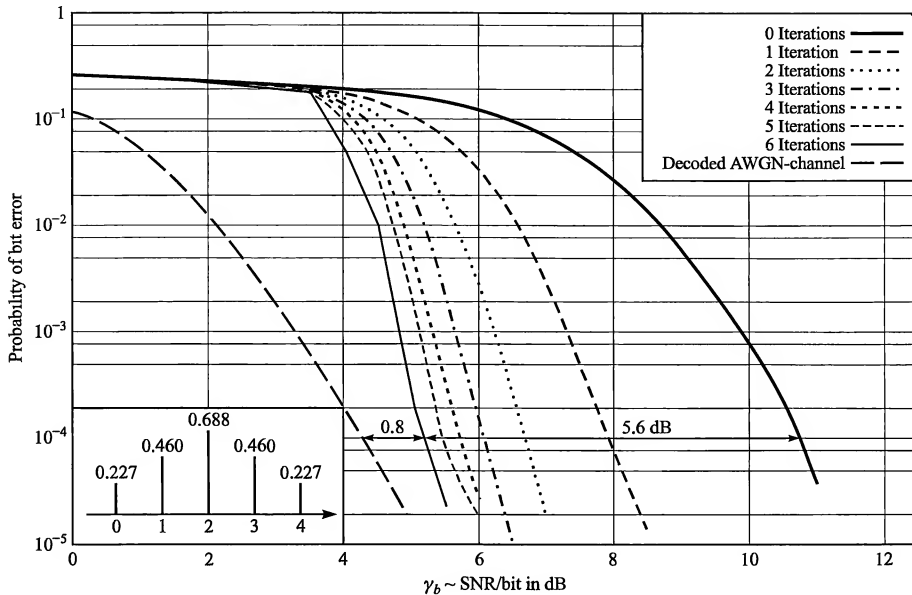
FIGURE 9.7-2 Channel taps and bit error rate for a time-invariant channel. [From Bauch et al. (1997).]
