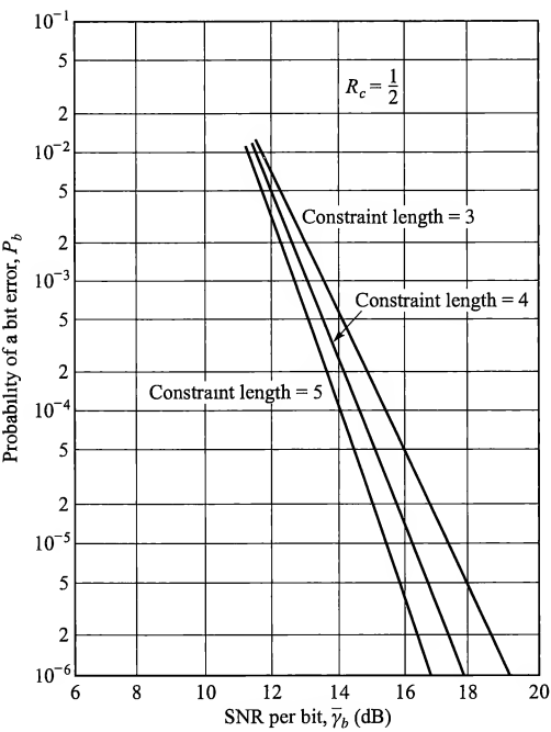
FIGURE 14.7-3 Performance of rate 1/2 binary convolutional codes with soft-decision decoding.
