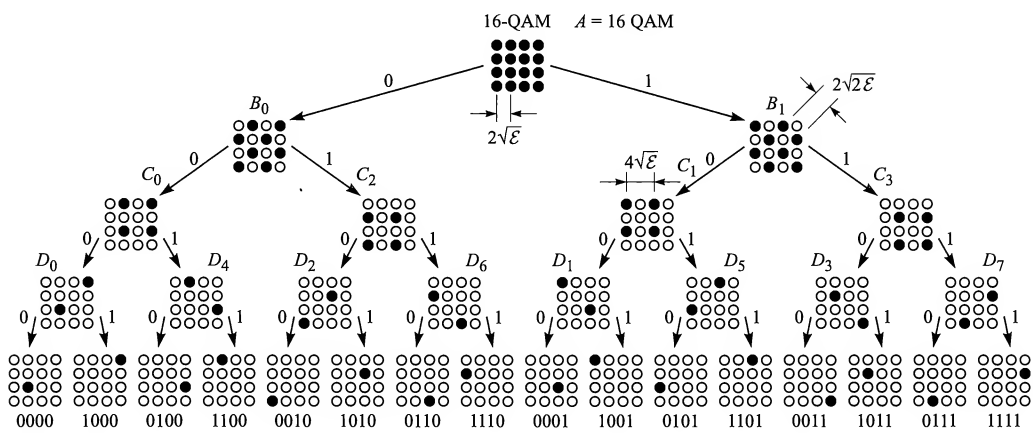
FIGURE 8.12-2 Set partitioning of 16-QAM signal.
