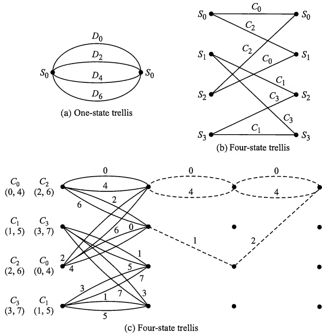
FIGURE 8.12-6 Uncoded 4-PSK and trellis-coded 8-PSK modulation.
