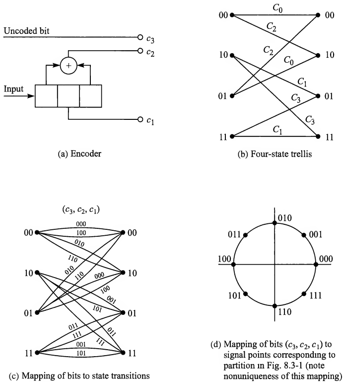
FIGURE 8.12-4 Four-state trellis-coded modulation with 8-PSK signal constellation.
