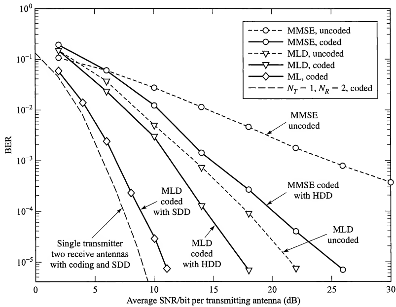
FIGURE 15.4-3 Performance of coded ( R_c = 1/2 , d_{\text{free}} = 5 ) systems with N_T = N_R = 2 .
