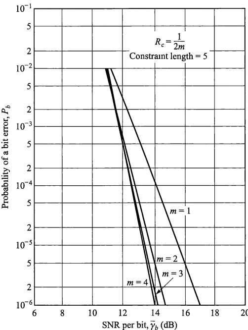
FIGURE 14.7-4 Performance of rate 1/2m , constraint length 5, binary convolutional codes with soft-decision decoding.
