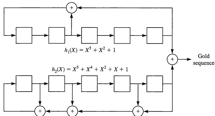
FIGURE 12.2-20 Generation of Gold sequences of length 31.
