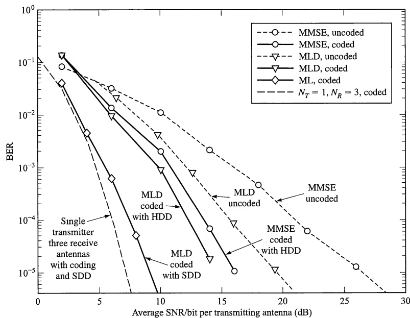
FIGURE 15.4-4 Performance of coded ( R_c = 1/2 , d_{\text{free}} = 5 ) systems with N_T = 2 , N_R = 3 .
