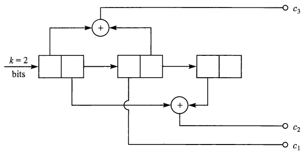
FIGURE 8.12-5 Rate \frac{2}{3} , eight-state trellis code.
