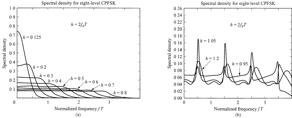
FIGURE 3.4-3 Power spectral density of octal CPFSK.
