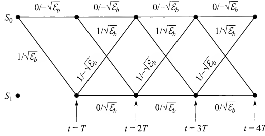
FIGURE 4.8-1 Trellis for NRZI signal.
