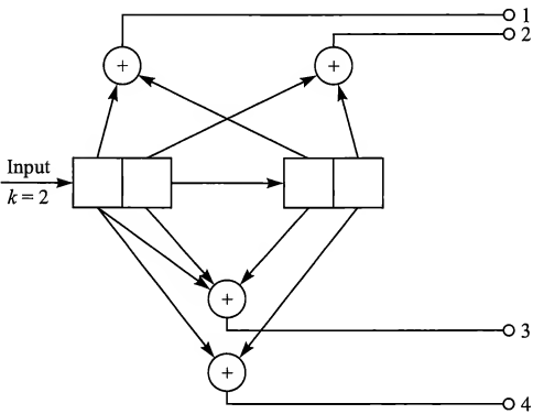
FIGURE 8.1–11 K = 2, k = 2, n = 4 convolutional encoder.
