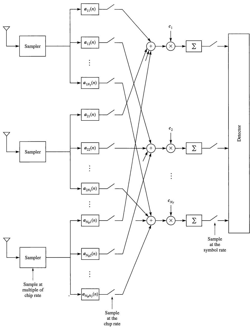
FIGURE 15.3–2 A MIMO receiver structure for a frequency-selective channel.
