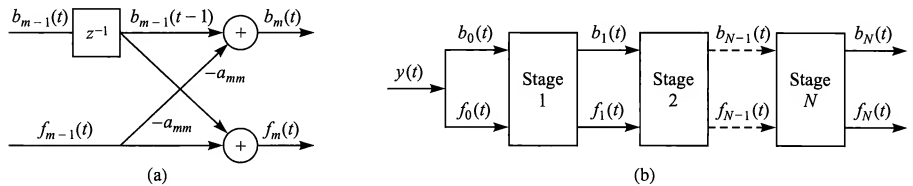
FIGURE 10.4-2 A lattice filter.
