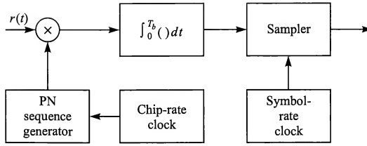
FIGURE 12.2-6 Correlation-type demodulator for a repetition code.
