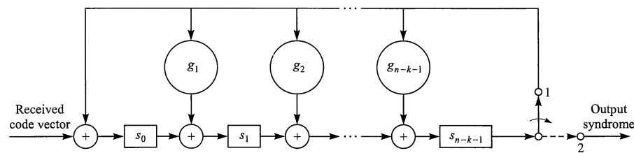
FIGURE 7.9-6 An (n - k) -stage shift register for computing the syndrome.
