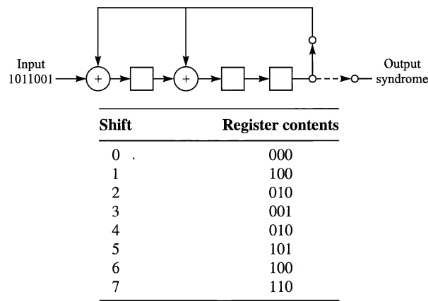
FIGURE 7.9-7 Syndrome computation for the (7, 4) cyclic code with generator polynomial g(X) = X^3 + X + 1 and received vector y = (1001101) .
