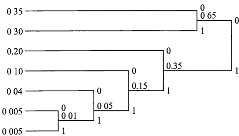
FIGURE 6.3-4 An example of variable-length source encoding for a DMS.
