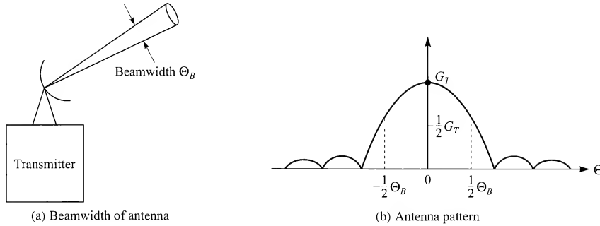
FIGURE 4.10-3 Antenna beamwidth and pattern.
