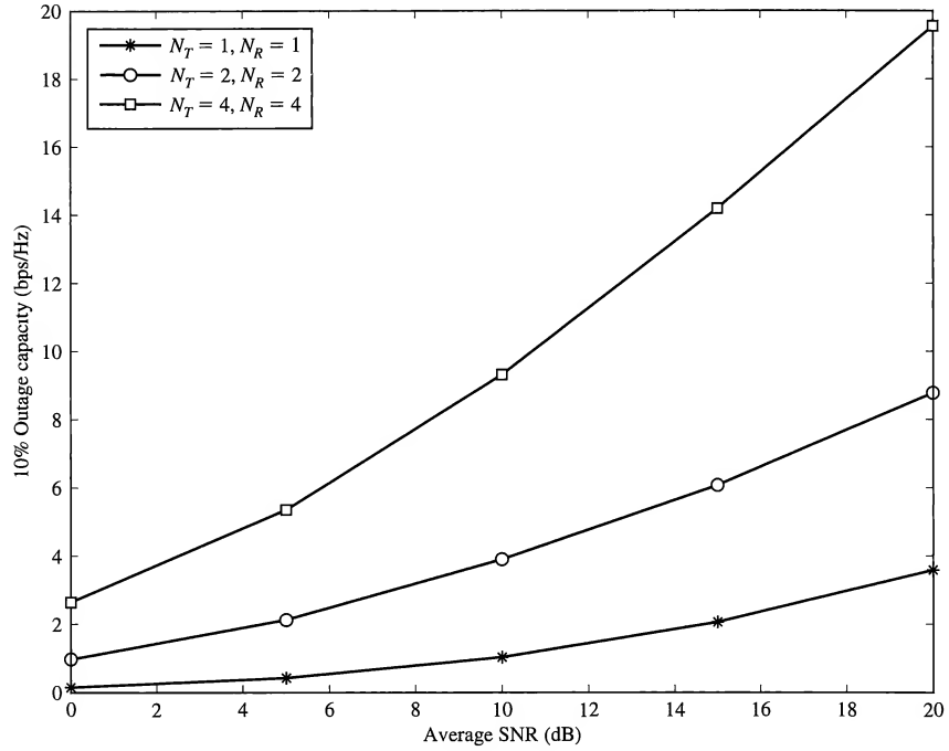
FIGURE 15.2-6 10% Outage capacity of MIMO channels.
