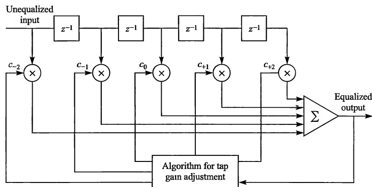
FIGURE 9.4–1 Linear transversal filter.
