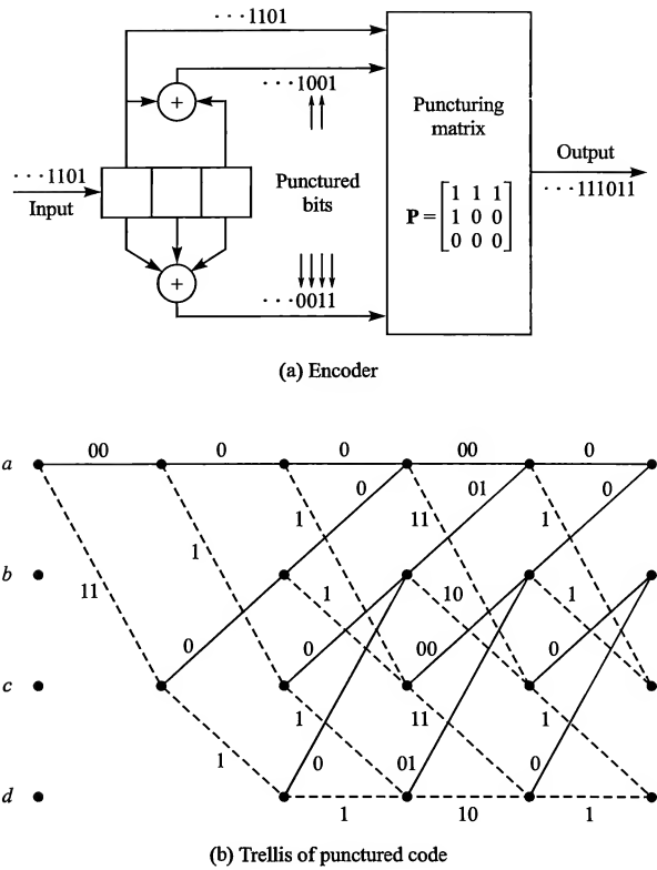
FIGURE 8.4-1 Generation of a rate 3/4 punctured code from a rate 1/3 convolutional code.
