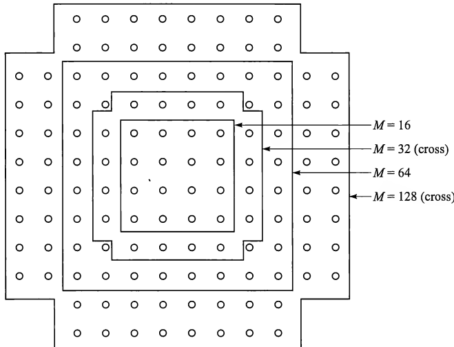
FIGURE 8.12–9 Rectangular two-dimensional (QAM) signal constellations.
