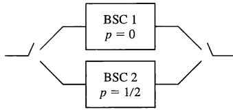
FIGURE 14.2–1 A two-state channel.
