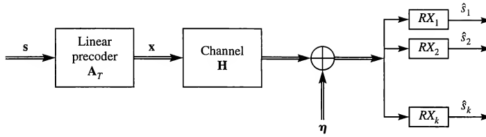
FIGURE 16.4–1 Model of MIMO broadcast system employing linear precoding.
