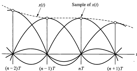
FIGURE 2.8-1 Sampling and reconstruction from samples.
