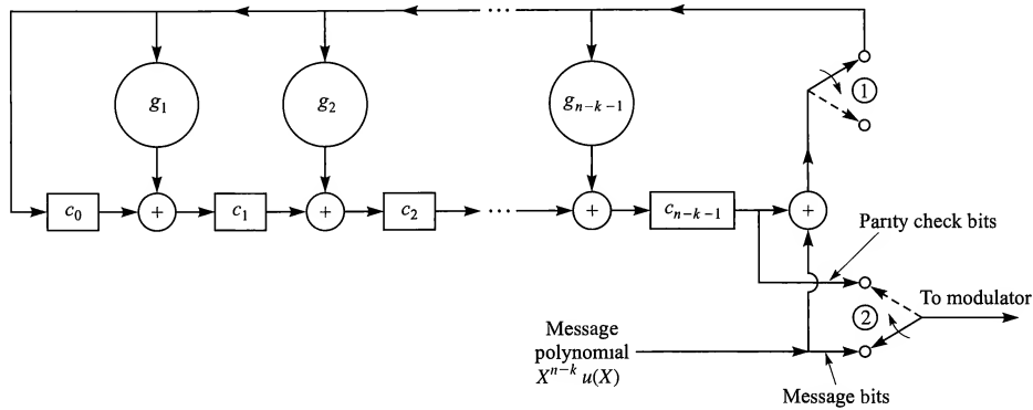
FIGURE 7.9-2 Encoding a cyclic code by use of the generator polynomial g(X) .
