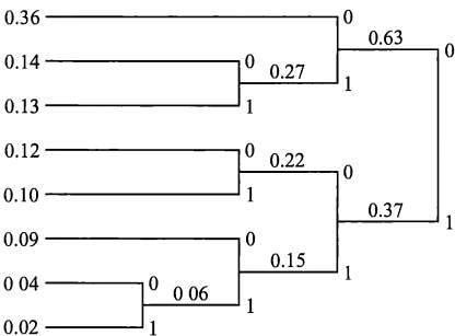
FIGURE 6.3-6 Huffman code for Example 6.3-2.
