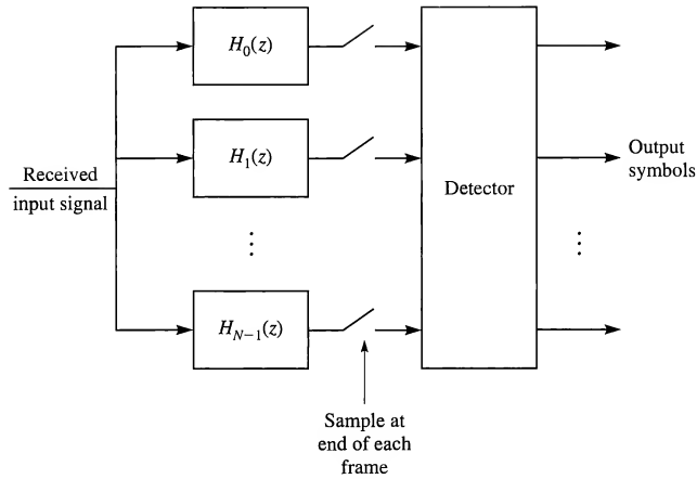
FIGURE 11.2–7 Filter bank implementation of OFDM receiver.
