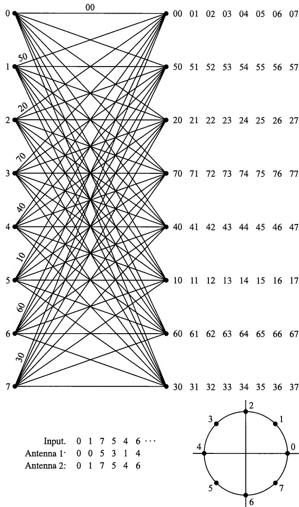
FIGURE 15.4-8 8-PSK, 8-state, space-time trellis code.
