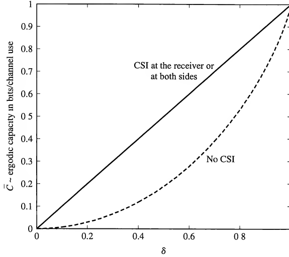
FIGURE 14.2-2 The ergodic capacity of channel model 1.
