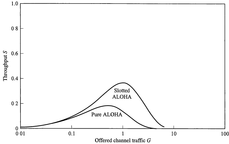
FIGURE 16.5-3 Throughput in ALOHA systems.
