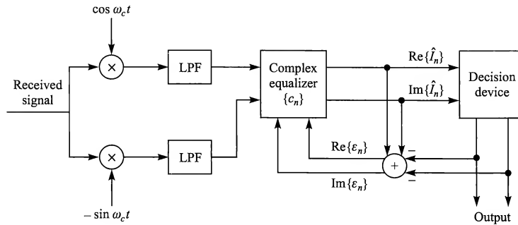
FIGURE 9.4-9 QAM and PSK signal demodulator with baseband equalizer.
