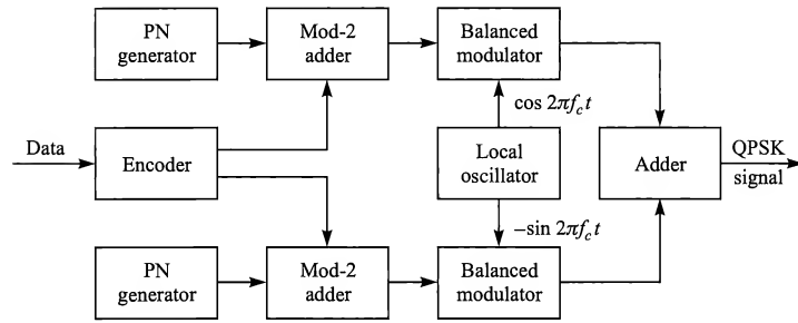
(b) DS-QPSK modulator
