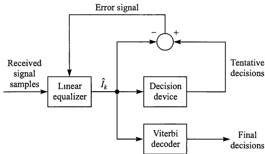
FIGURE 10.3-1 Adjustment of equalizer based on tentative decisions.
