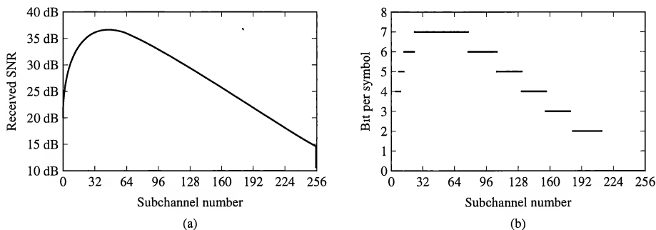
FIGURE 11.2–9 Example of a DSL frequency response and bit allocation on the OFDM subchannels.
