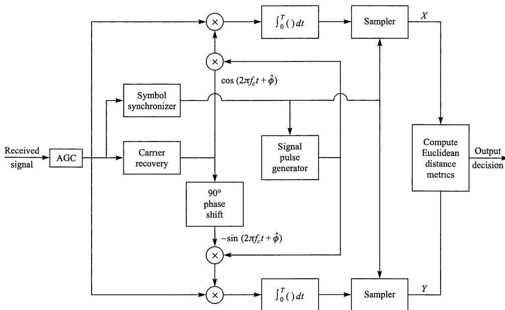
FIGURE 5.1–4 Block diagram of a QAM receiver.
