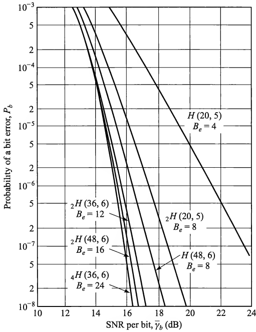
FIGURE 14.7-5 Performance of Hadamard codes.
