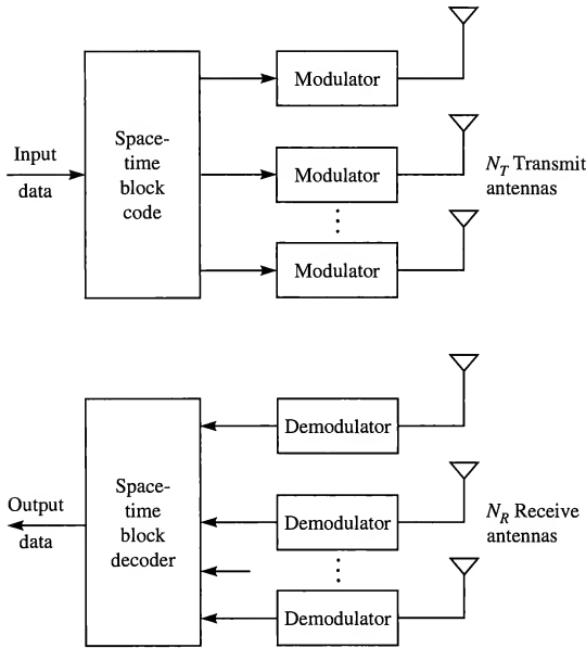
FIGURE 15.4-5 Space-time block coded MIMO system.
