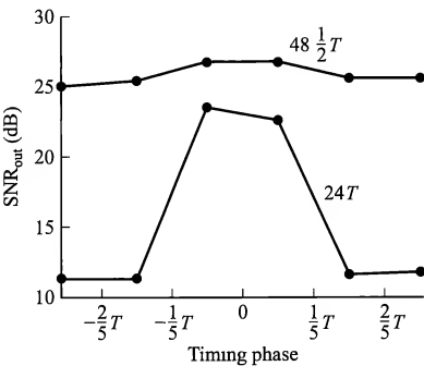
FIGURE 9.4-8 Performance of T and \frac{1}{2} T equalizers as a function of timing phase for 2400 symbols/s 16-QAM on a channel with poor envelope delay. [From Gitlin and Weinstein (1981). Reprinted with permission from Bell System Technical Journal. © 1981 AT & T.]
