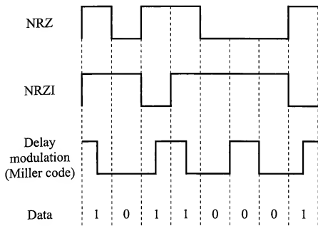
FIGURE 3.3-1 Examples of baseband signals.
