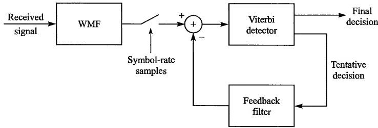
(a) Block diagram of symbol detector
