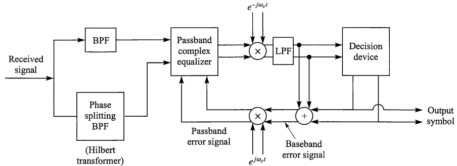
FIGURE 9.4–11 QAM or PSK signal equalization at passband.
