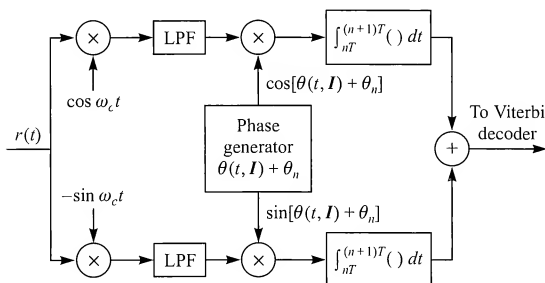
FIGURE 4.9-4 Computation of metric increments v_n(\mathbf{I}; \theta_n) .
