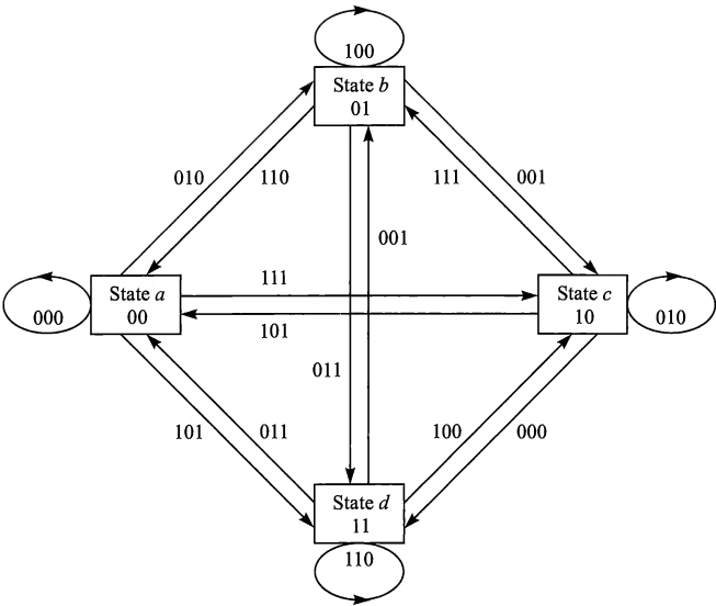
FIGURE 8.1–10 State diagram for K = 2, k = 2, n = 3 convolutional code.
