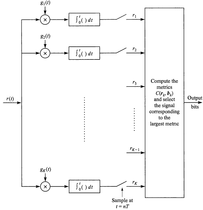
FIGURE 16.3-1 Optimum multiuser receiver for synchronous transmission.
