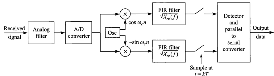
(b) QAM or PSK demodulator
