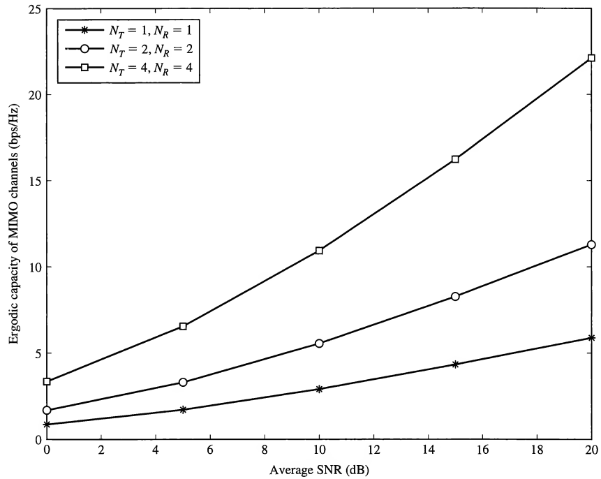
FIGURE 15.2-3 Ergodic capacity of MIMO channels.
