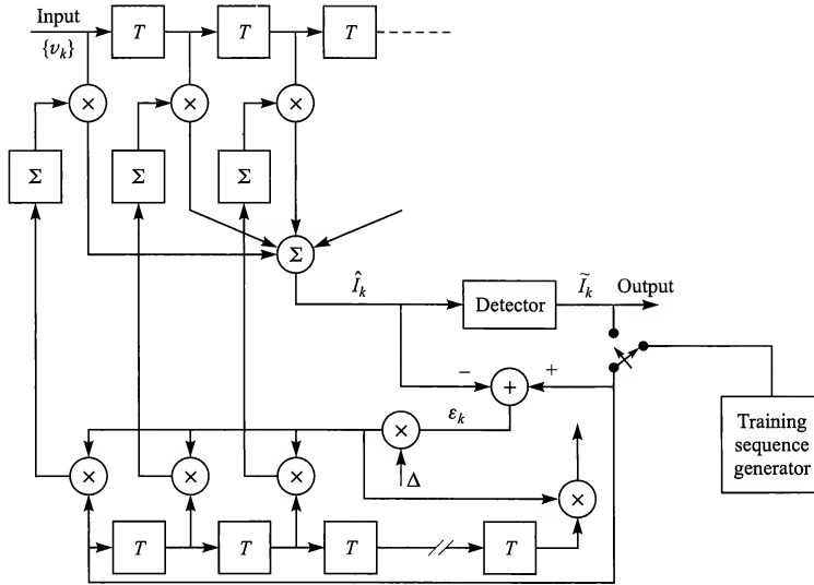
FIGURE 10.1-1 An adaptive zero-forcing equalizer.
