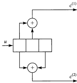
FIGURE 8.1-17 A catastrophic convolutional encoder.
