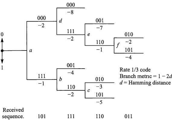
FIGURE 8.5–3 An example of the stack algorithm for decoding a rate 1/3 convolutional code.
