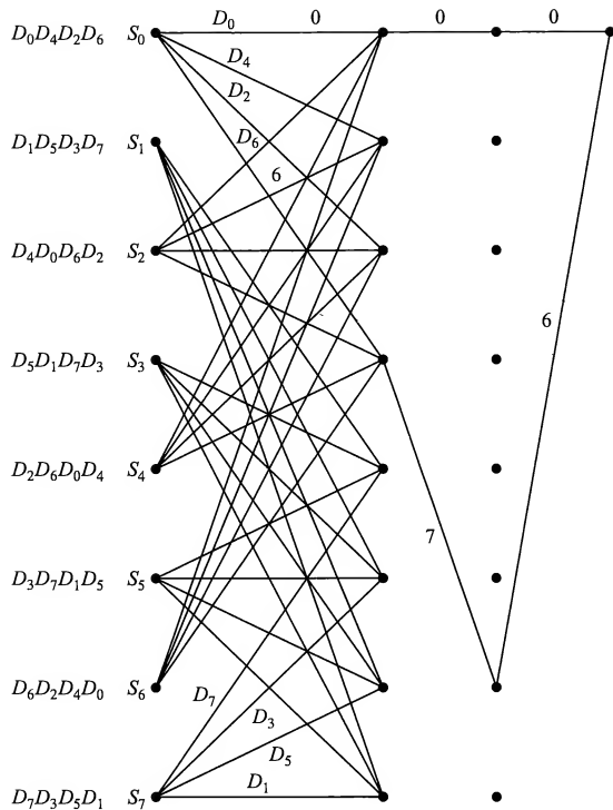
FIGURE 8.12-8 Eight-state trellis code for coded 8-PSK modulation.
