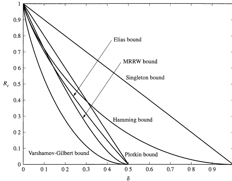
FIGURE 7.7-1 Comparison of Asymptotic Bounds.
