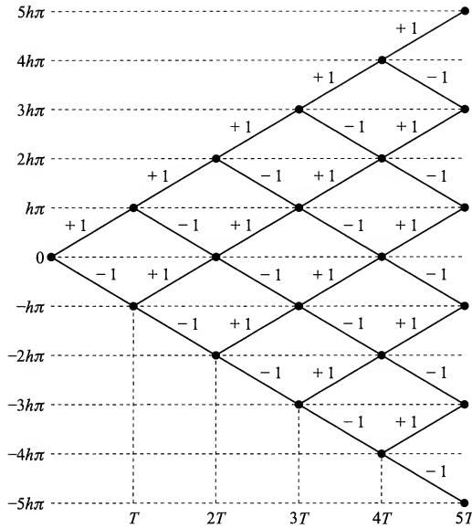
FIGURE 3.3-5 Phase trajectory for binary CPFSK.
