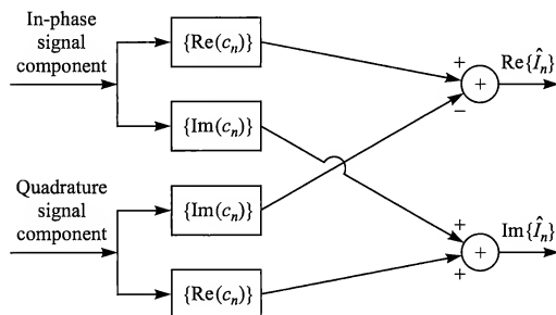
FIGURE 9.4-10 Complex-valued baseband equalizer for QAM and PSK signals.
