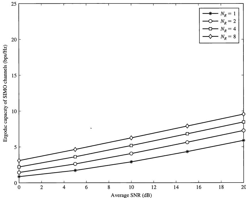
FIGURE 15.2–1 Ergodic capacity of SIMO channels.
