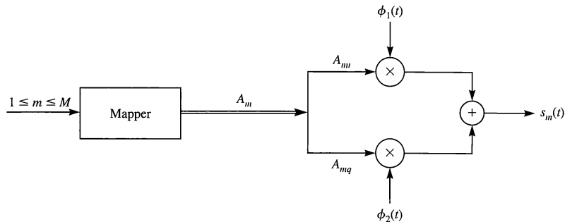
FIGURE 3.2-6 A general QAM modulator.
