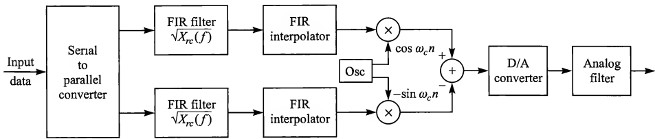
(a) QAM or PSK modulator
