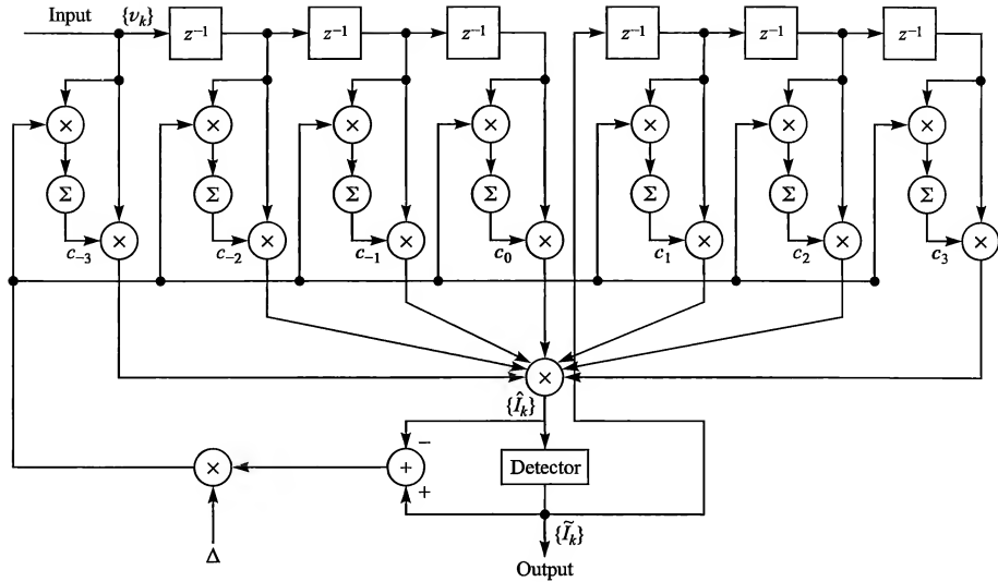
FIGURE 10.2–1 Decision-feedback equalizer.
