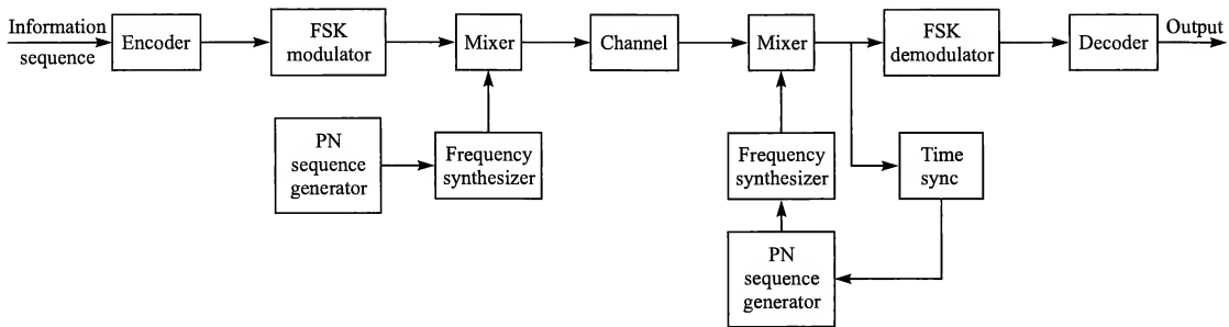
FIGURE 12.3-2 Block diagram of an FH spread spectrum system.
