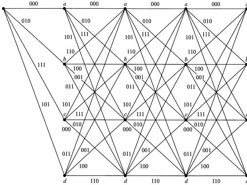
FIGURE 8.1-9 Trellis diagram for K = 2, k = 2, n = 3 convolutional code.
