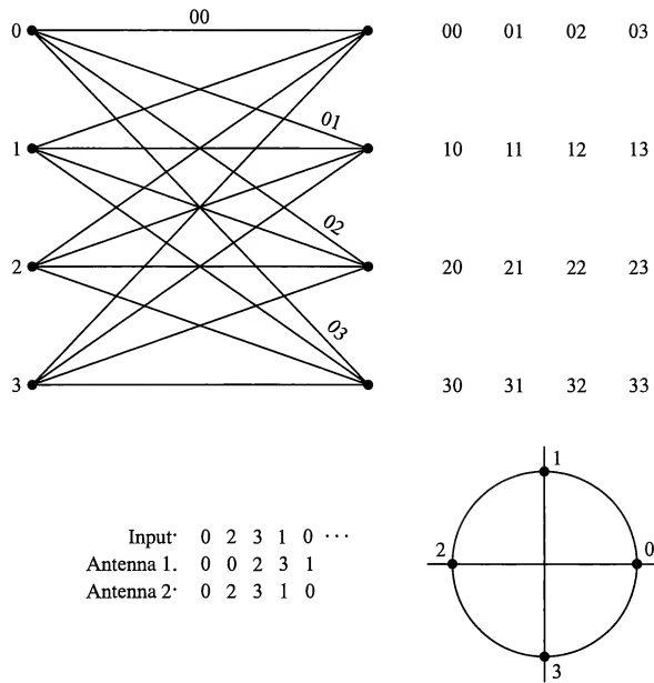
FIGURE 15.4-6 4-PSK, 4-state, space-time trellis code.
