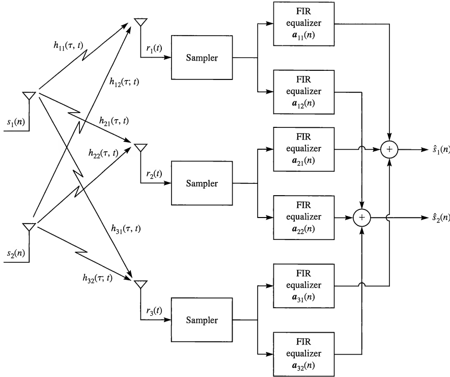
FIGURE 15.1–6 Signal demodulation with linear equalizers for the frequency-selective channel.
