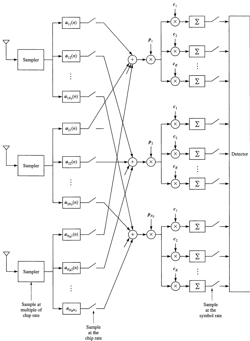
FIGURE 15.3-5 Receiver structure for a MIMO multicode system in a frequency-selective MIMO channel.
