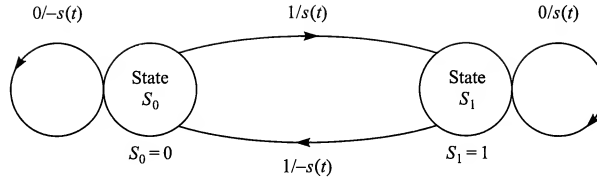
FIGURE 3.3-2 State transition diagram for NRZI signaling.
