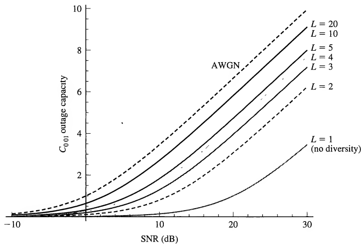
FIGURE 14.2–8 The outage capacity of fading channels with different diversity orders.
