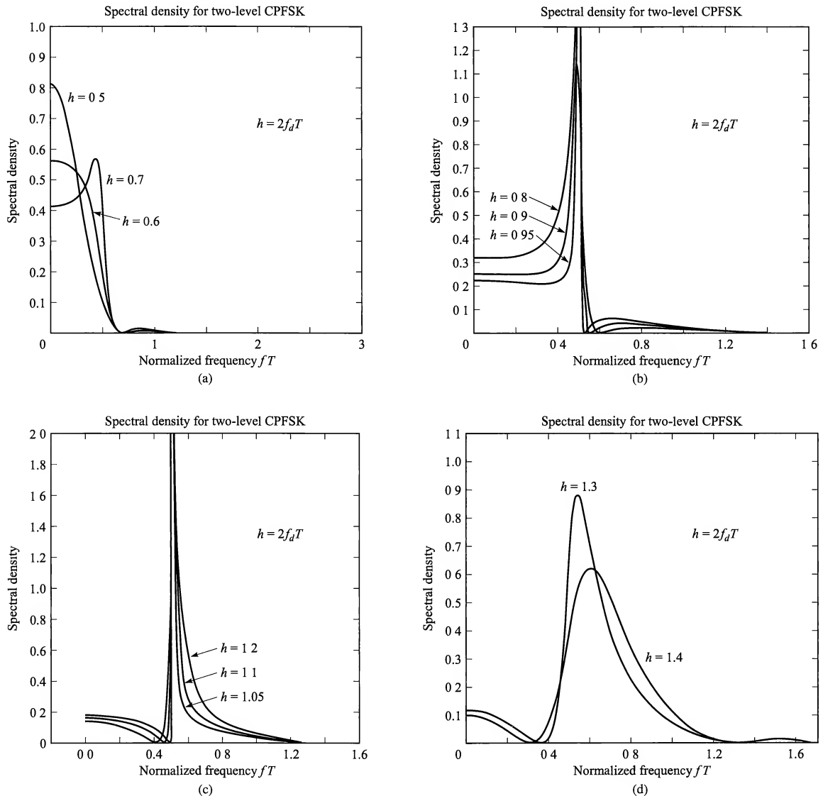
FIGURE 3.4-1 Power spectral density of binary CPFSK.
