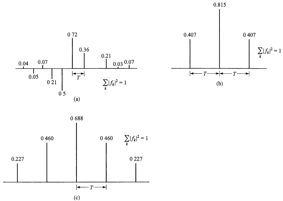
FIGURE 9.4-5 Three discrete-time channel characteristics.
