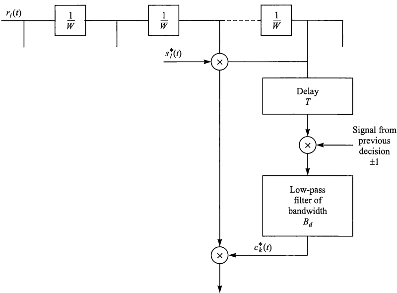
FIGURE 13.5–5 Channel tap weight estimation with binary antipodal signals.
