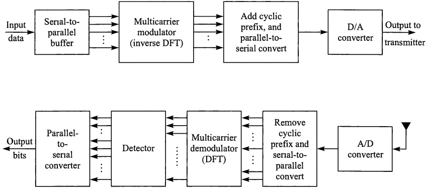
FIGURE 11.2-4 Multicarrier communication system.
