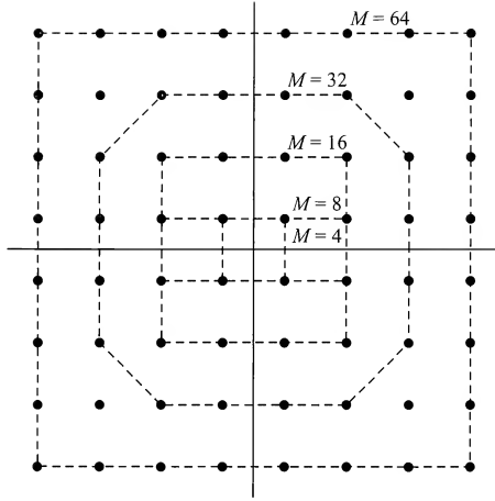
FIGURE 4.7-2 QAM constellation.
