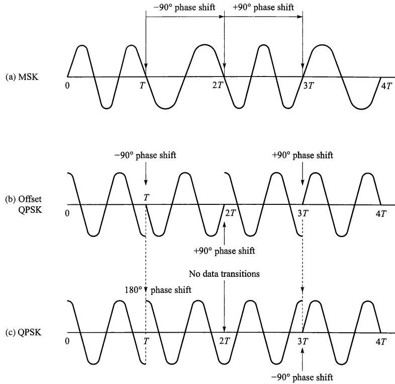
FIGURE 3.3-17 MSK, OQPSK, and QPSK signals.
