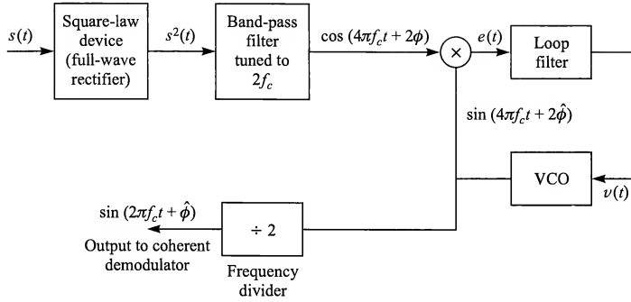
FIGURE 5.2–14 Carrier recover using a square-law device.
