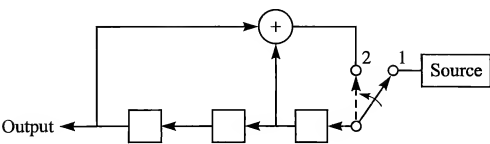
FIGURE 7.9-8 Three-stage ( m = 3 ) shift register with feedback.
