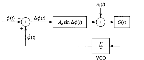
FIGURE 5.2-6 Equivalent PLL model with additive noise.
