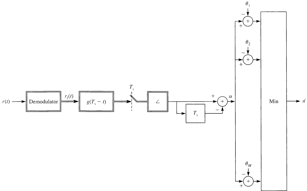
FIGURE 4.5-4 The DPSK receiver.
