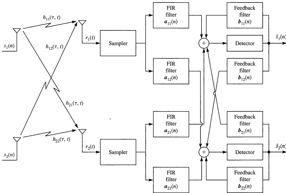
FIGURE 15.1–8 Signal demodulation with decision-feedback equalizers for the frequency-selective channel.
