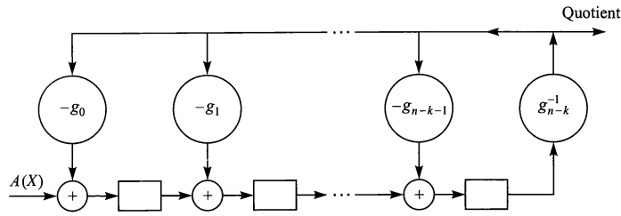
FIGURE 7.9-1 A feedback shift register for dividing the polynomial A(X) by g(X) .
