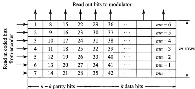
FIGURE 7.12–2 A block interleaver for coded data.
