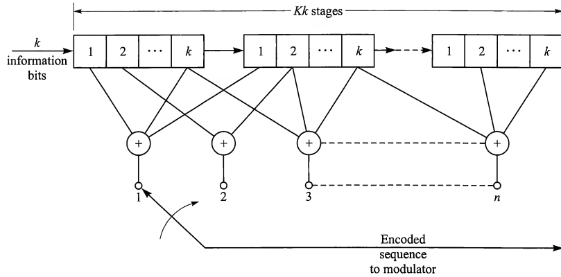
FIGURE 7.1-1 A convolutional encoder.
