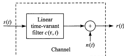
FIGURE 1.3-3 Linear time-variant filter channel with additive noise.
