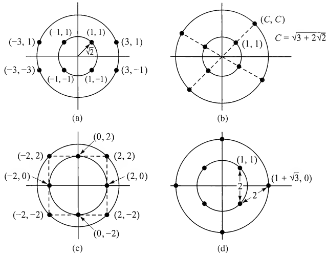
FIGURE 4.3-7 Four eight-point signal constellations.
