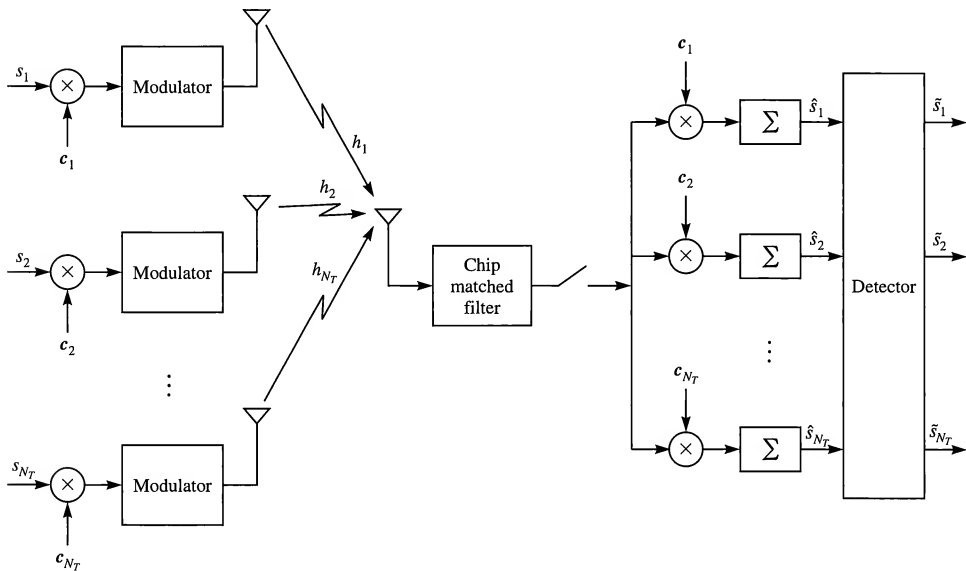
FIGURE 15.3–3 MISO system with spread spectrum signals.
