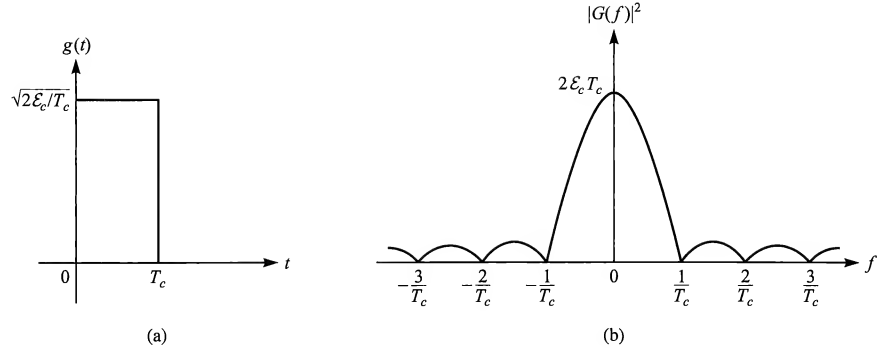
FIGURE 12.2-3 Rectangular pulse and its energy density spectrum.
