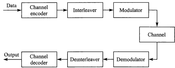
FIGURE 7.12–1 Block diagram of system employing interleaving for burst error channel.
