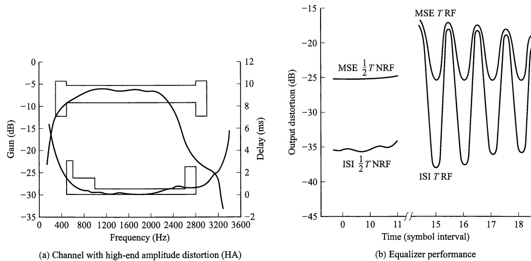
FIGURE 9.4-7 T and \frac{1}{2} T equalizer performance as a function of timing phase for 2400 symbols per second. (NRF indicates no receiver filter.) [From Qureshi and Forney (1977). © 1977 IEEE.]
