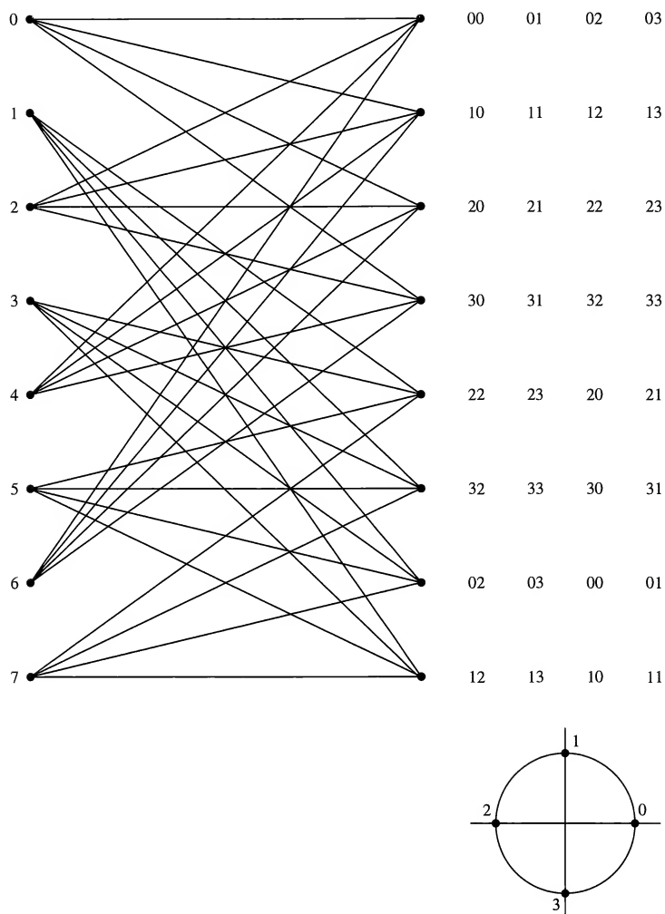
FIGURE 15.4-7 4-PSK, 8-state, space-time trellis code.
