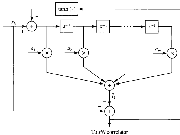
FIGURE 12.2-18 Non-linear excision filter.
