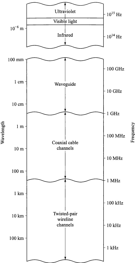
FIGURE 1.2-1 Frequency range for guided wire channel.
