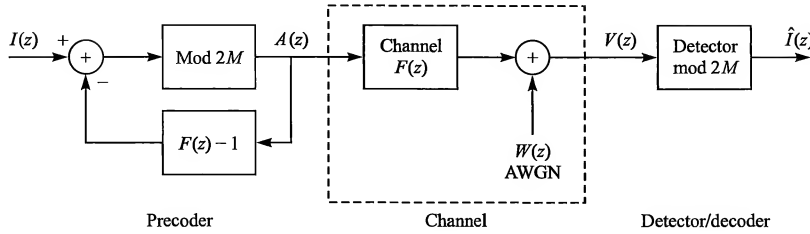
FIGURE 9.5–5 Tomlinson–Harashima precoding.
