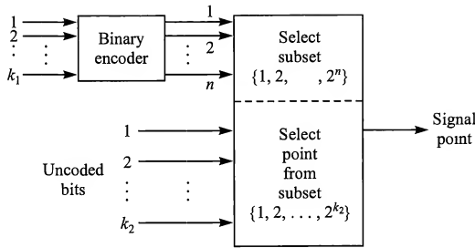
FIGURE 8.12-3 General structure of combined encoder/modulator.
