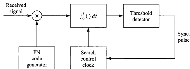
FIGURE 12.5-1 A sliding correlator for DS signal acquisition.
