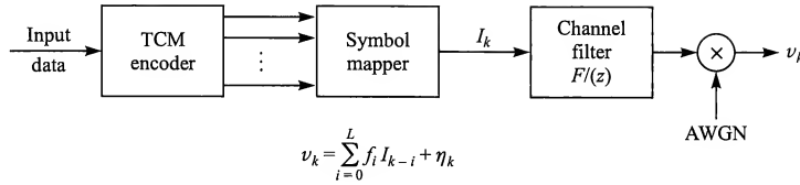
FIGURE 10.3–4 Model of TCM and ISI channel.
