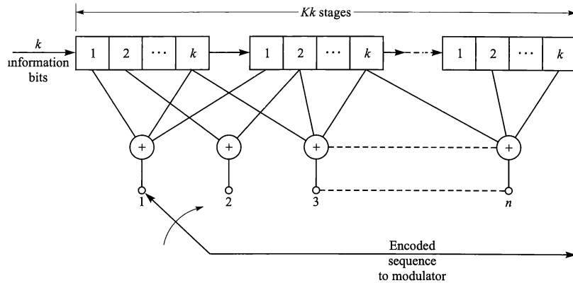
FIGURE 8.1-1 Convolutional encoder.
