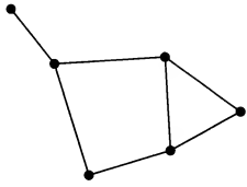
FIGURE 8.10-1 An example of a graph.
