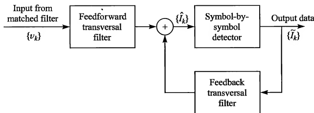
FIGURE 9.5–1 Structure of decision-feedback equalizer.
