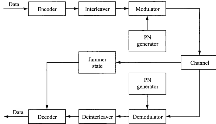
FIGURE 12.2–10 Block diagram of AJ communication system.
